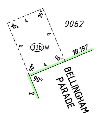
ENLARGEMENT 'L1' SCALE 1:200
