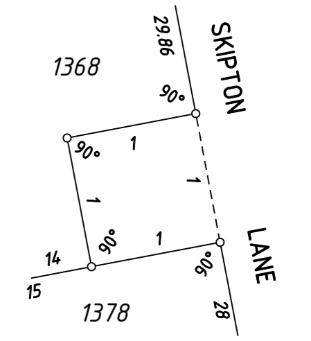
ENLARGEMENT 'E' SCALE 1:40
