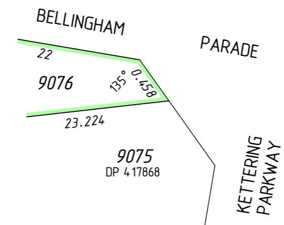
ENLARGEMENT 'B1' Not to scale
