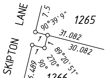
ENLARGEMENT 'B5' Not to Scale
