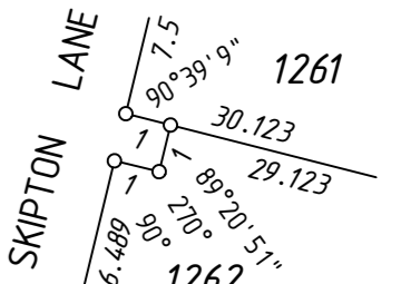
ENLARGEMENT 'B4' Not to Scale
