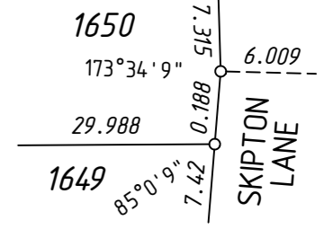
ENLARGEMENT 'B2' Not to Scale
