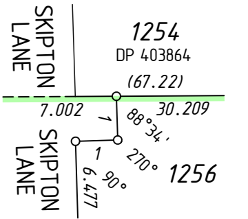
ENLARGEMENT 'B3' Not to Scale
