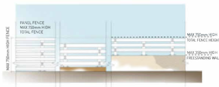
WALL & FENCE DETAIL HORIZONTAL SLATS
