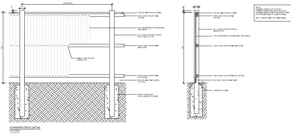
STANDARD FENCE DETAIL ELEVATION SCALE: 1:10
