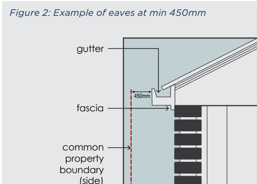
Figure 2: Example of eaves at min 450mm
