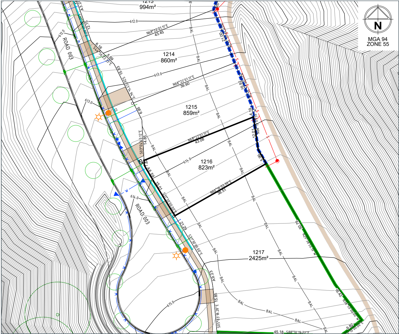
LOT LAYOUT - SCALE 1:400 (A4)
