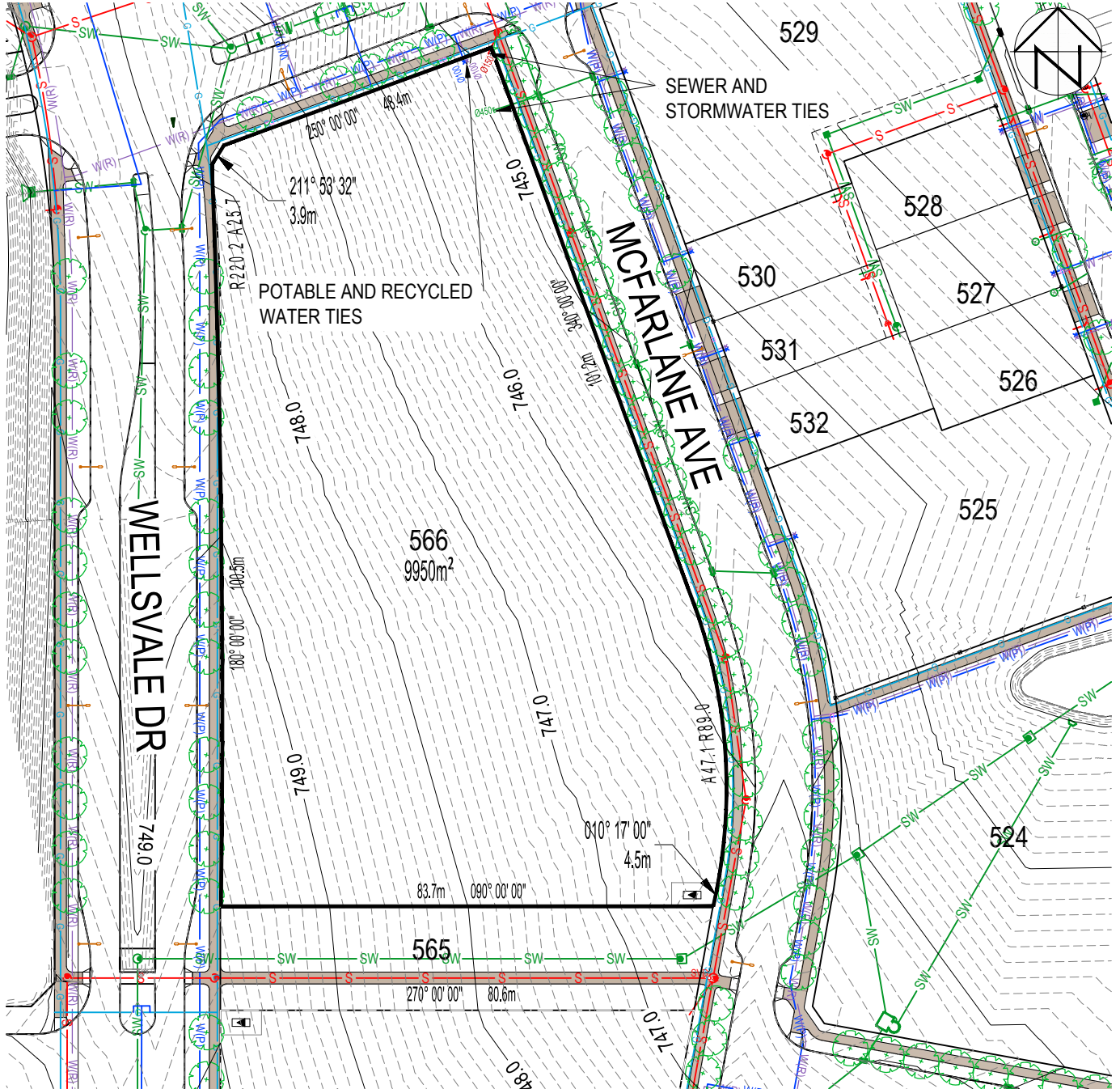
LOT LAYOUT - SCALE 1:1000
